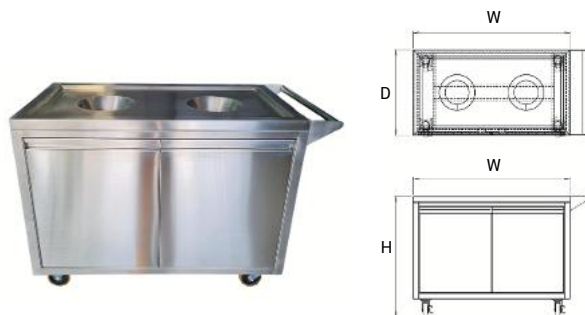
Food Waste Cleaning Trolley
