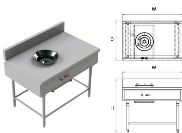
1-Burner Thai Range
