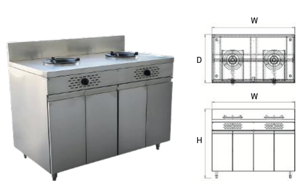
2-Stock Pot Stove Low Pressure
