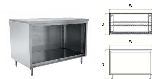
Open Cabinet
