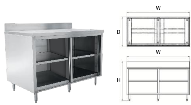
Open Cabinet With Under Shelf And Backsplash
