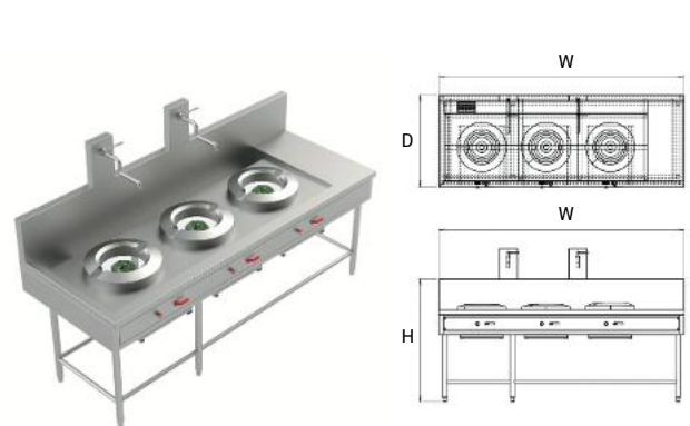
3-Burner Chinese Range With Faucet
