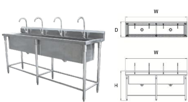
Sink Table With 4 Faucets And Backsplash
