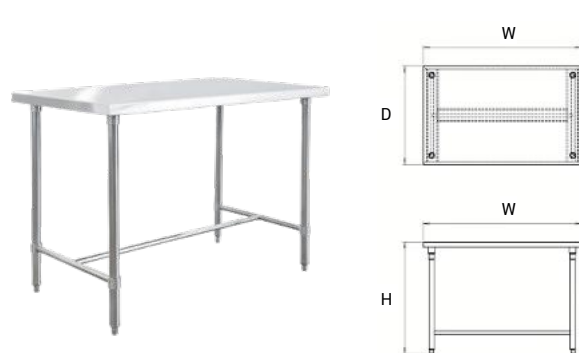
Work Table
