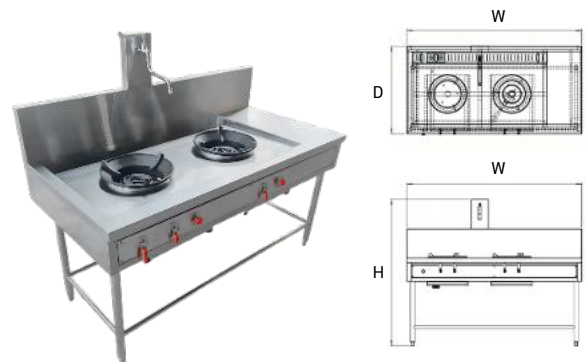
2-Burner Thai Range With Faucet
