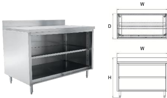
Open Cabinet With Under Shelf And Backsplash
