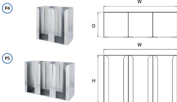
2-3 Cup Holders
