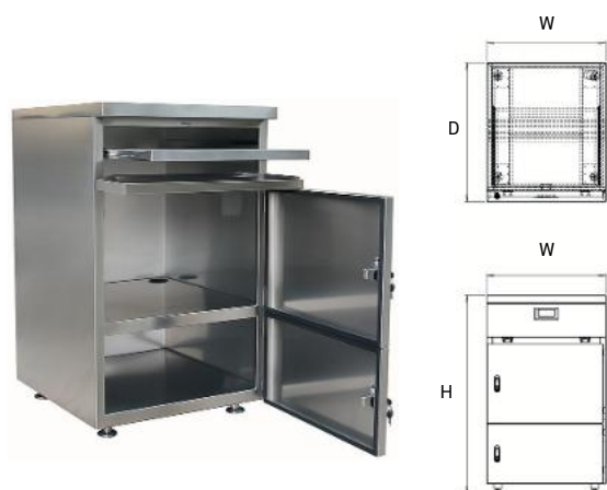
Custom Cabinet
