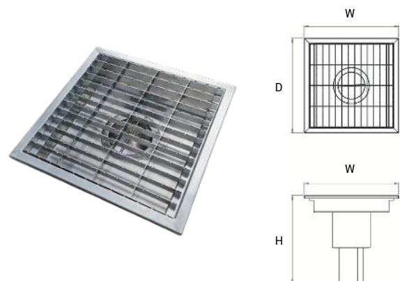
Gutter Stainless Steel
