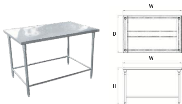
Work Table
