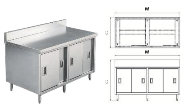
Cabinet Sliding Doors And Backsplash
