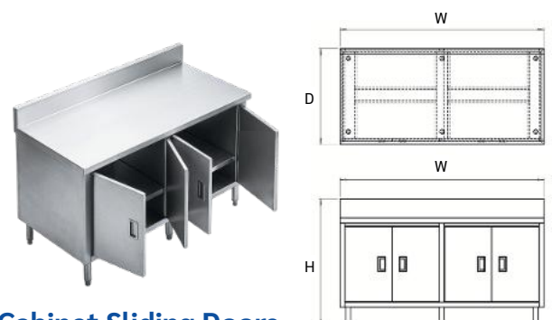
Cabinet Sliding Doors With Under Shelves And Backsplash
