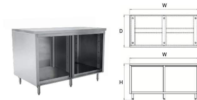
Open Cabinet
