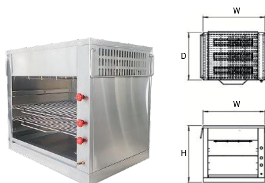
3-Burner Saramander Grill
