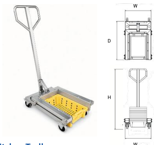
Kitchen Trolley
