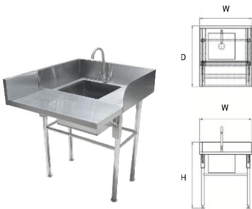
Foldable Side Sink With Backsplash
