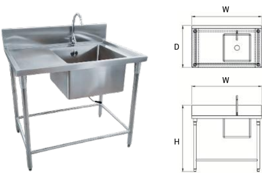
Sink Table With Faucet And Backsplash
