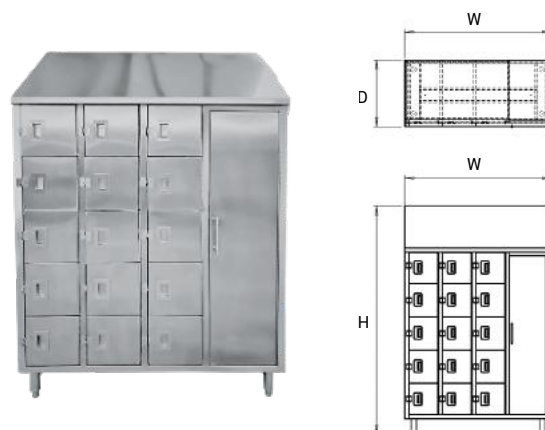
Multi-Purpose Cabinet
