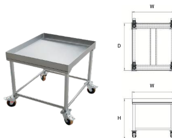
Product Trolley
