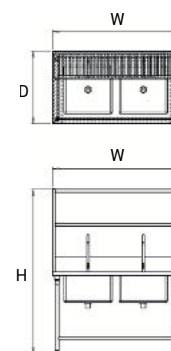
2 - Sink Table With Backsplash And Shelf
