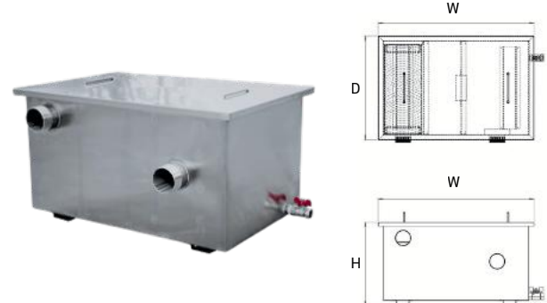
Grease Trap
