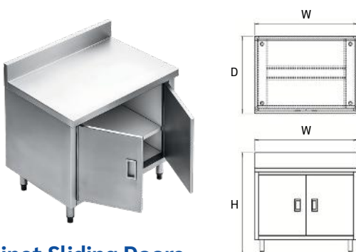
Cabinet Sliding Doors With Under Shelves And Backsplash
