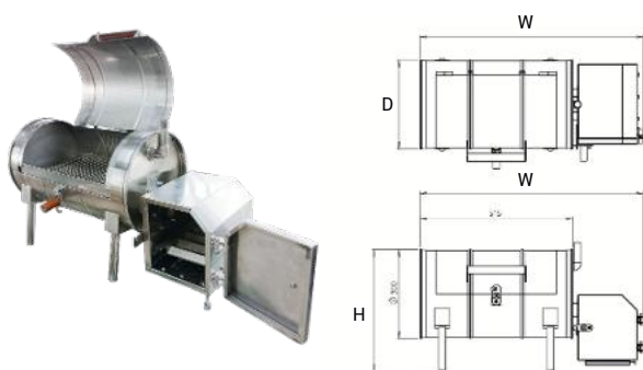
Smoke Oven
