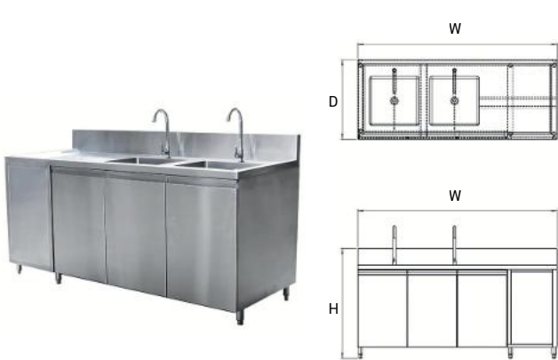
Sink Cabinet With 2 Faucets And Backsplash
