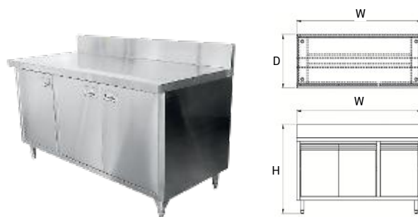
Cabinet Swing Doors With Backsplash
