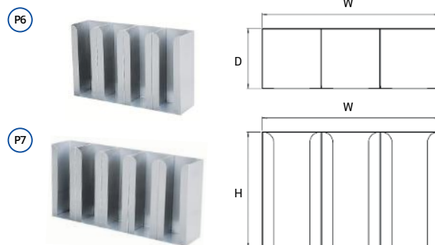
4-5 Cup Holders
