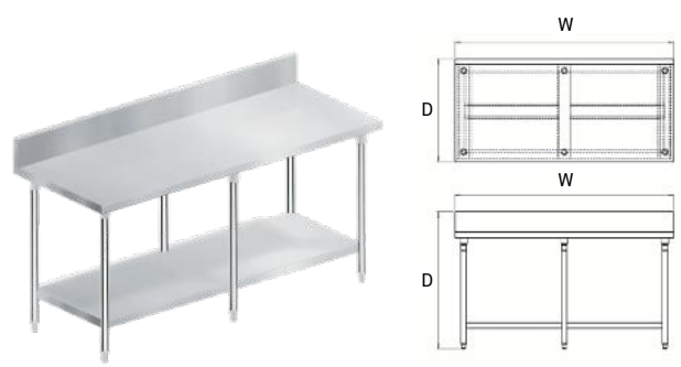
Work Table With Undershelf And Backsplash
