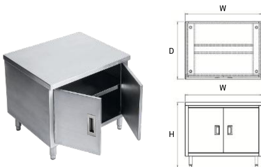
Cabinet Sliding Doors With Under Shelves
