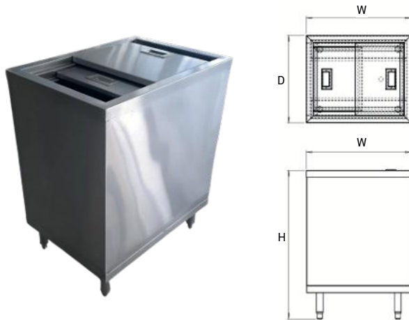
Ice Bin Cabinet
