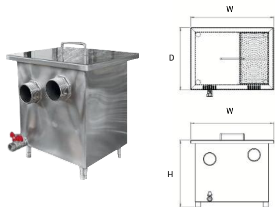
Grease Trap
