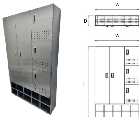
Multi-Purpose Cabinet
