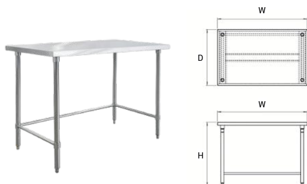
Work Table
