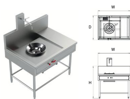
1-Burner Thai Range With Faucet
