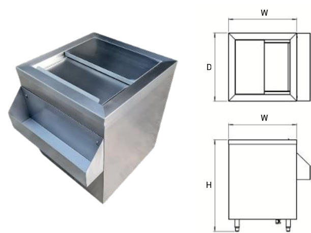
Ice Bin Cabinet
