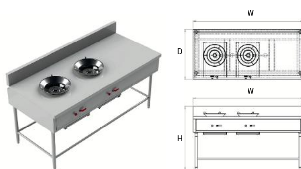
2-Burner Thai Range
