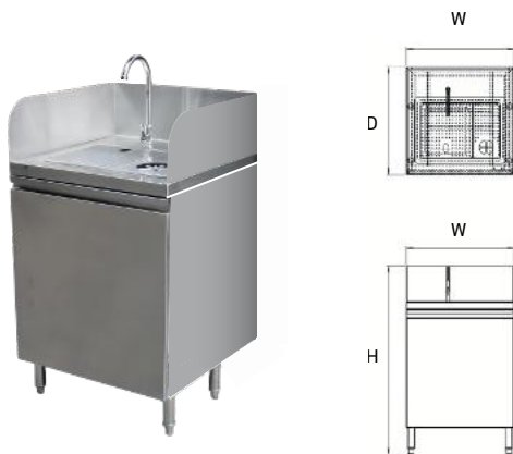
Glass Rinser Kitchen Sink
