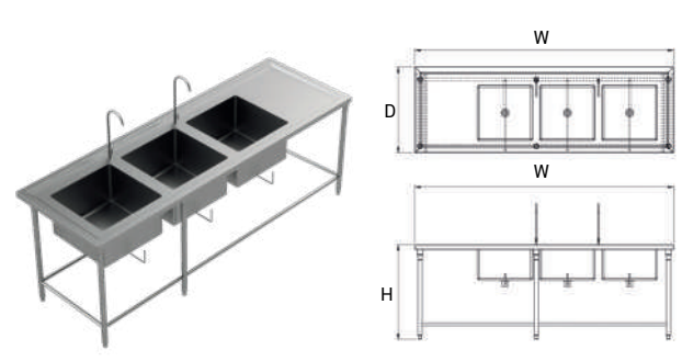
Triple Sink Table With 2 Faucets
