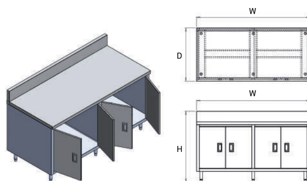
Cabinet Swing Doors With Backsplash
