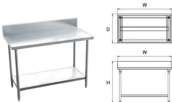
Work Table With Undershelf And Backsplash
