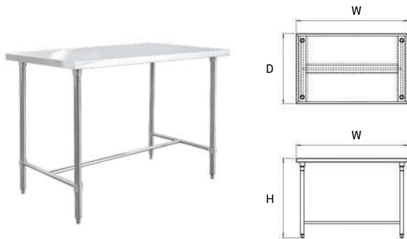
Work Table
