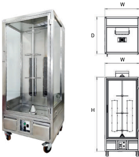
1-Grill Machine
