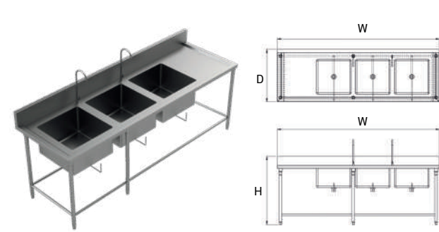
Triple Sink Table With 2 Faucets And Backsplash
