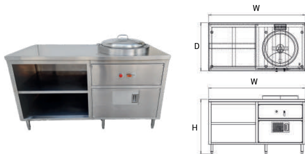
Right - Noodle Range
