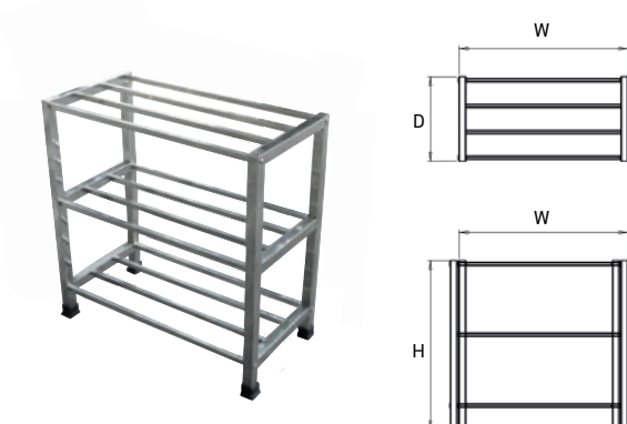
Stainless Steel Shoe Rack
