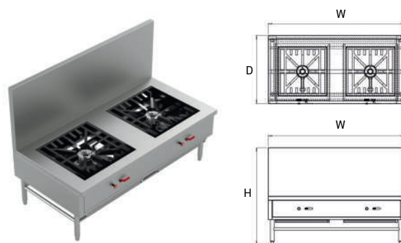
2-Stock Pot Stove High Pressure
