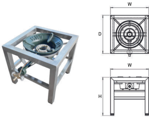
Thai Gas Burner With Stand
