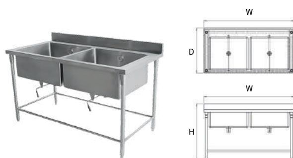
2 - Sink Table With Backsplash
