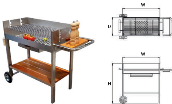
BBQ Grill Trolley
