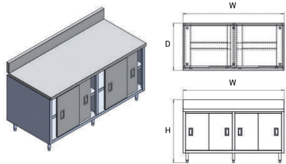
Cabinet Sliding Doors With Under Shelf And Backsplash
