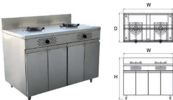
2-Stock Pot Stove Low Pressure
