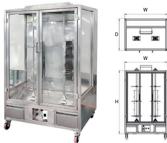
2-Grill Machine
