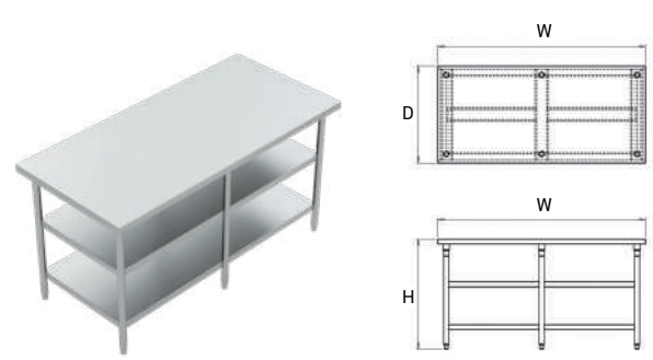
Work Table With Double Under Shelves
