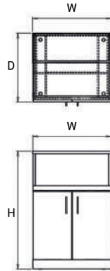
Cabinet With Front Doors + Extra Shelf
