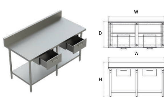
Work Table With Under Shelf Drawers And Backsplash
