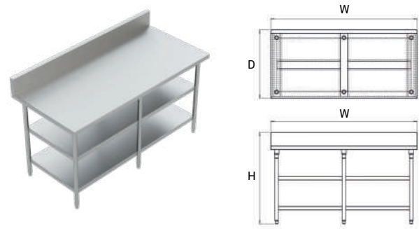
Work Table With Double Under Shelves And Backsplash
