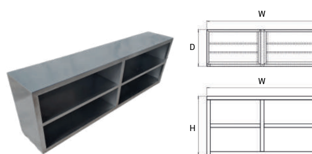
Open Wall Cabinet With Under Shelf
