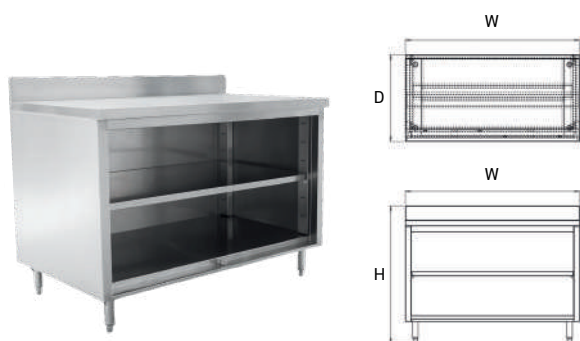
Open Cabinet With Under Shelf And Backsplash
