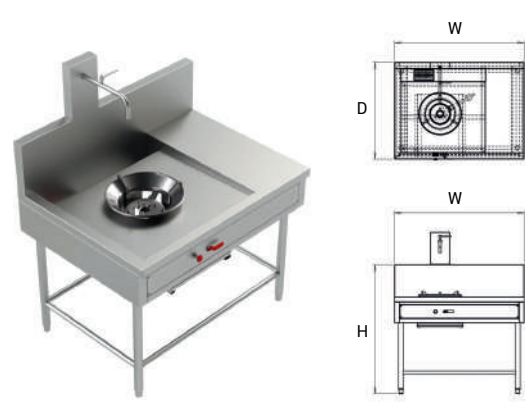
1-Burner Thai Range With Faucet
