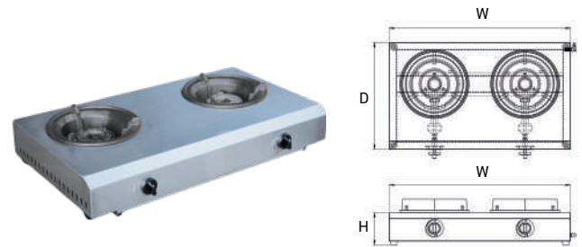
2 - Gas Stove Table
