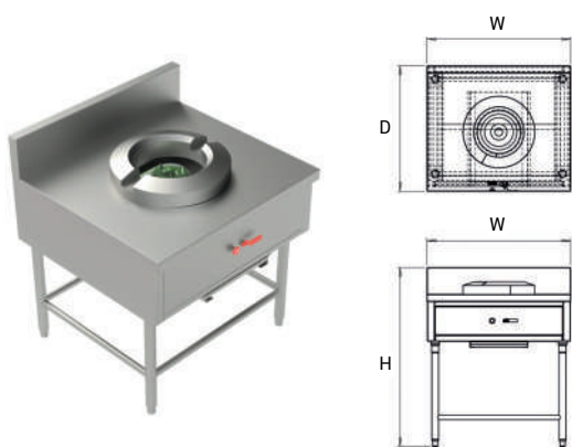
1-Burner Chinese Range
