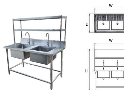
2 - Sink Table With Backsplash And Shelf
