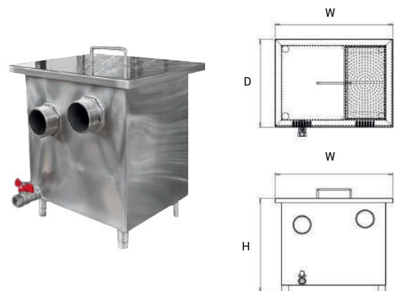
Grease Trap
