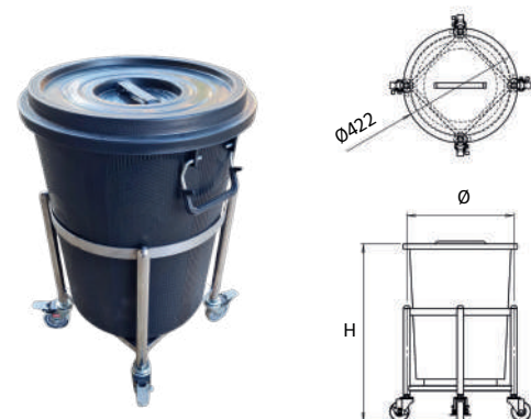
Mobile Garbage Bin
