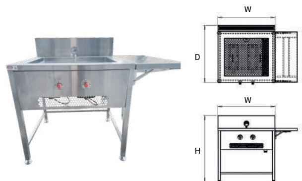
Deep Fryer For Dough Sticks
