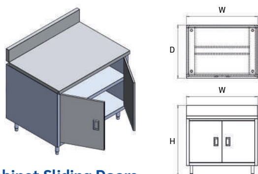
Cabinet Sliding Doors With Under Shelves And Backsplash
