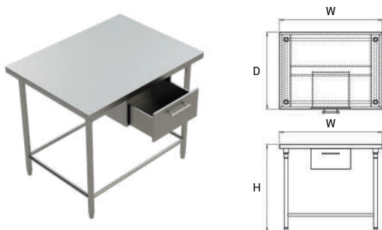
Work Table With Drawers
