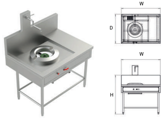
1-Burner Chinese Range With Faucet
