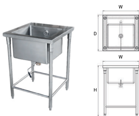
1 - Sink Table
