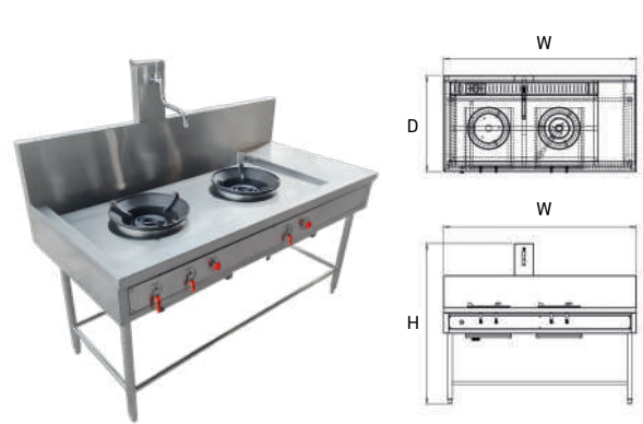
2-Burner Thai Range With Faucet
