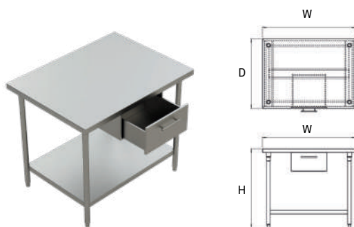
Work Table With Under Shelf And Drawers
