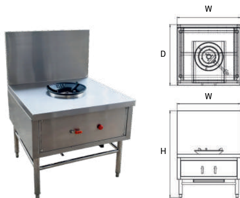
1-Stock Pot Stove Low Pressure
