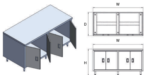
Cabinet Swing Doors
