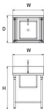
Sink Table With Faucet And Backsplash
