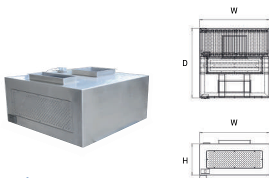
Hood
