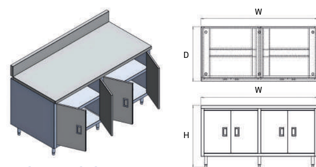
Cabinet Sliding Doors With Under Shelves And Backsplash
