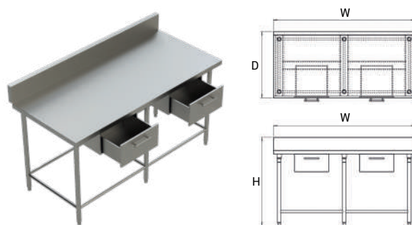
Work Table With Drawers And Backsplash
