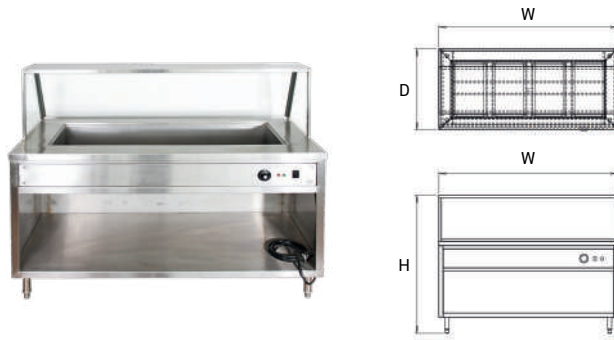
Food Warmer
