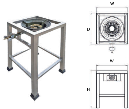
Thai Gas Burner With Stand
