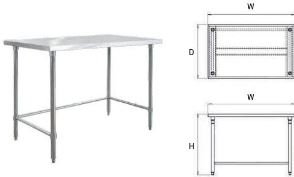
Work Table
