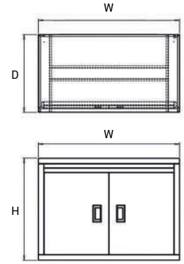
Cabinet Sliding Doors With Under Shelves
