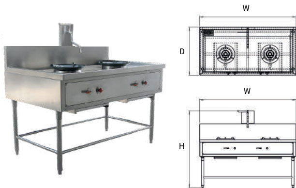
2-Burner Thai Range With Faucet
