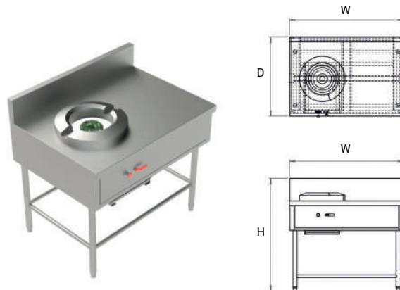
1-Burner Chinese Range
