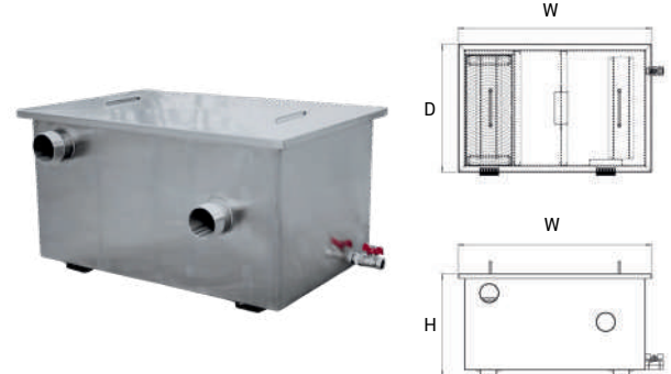
Grease Trap
