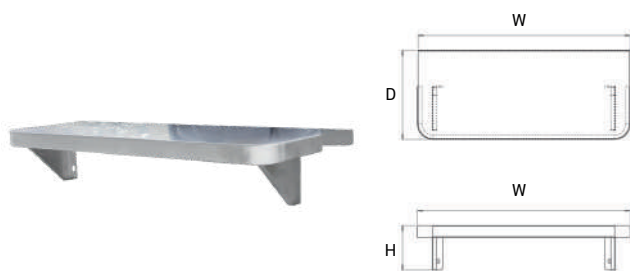
Wall Shelf
