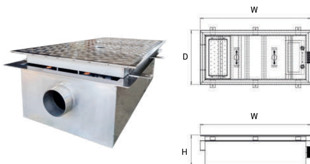
Drainage Trench Stainless
