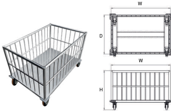
Cage Trolley
