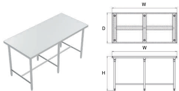
Work Table
