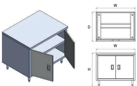
Cabinet Sliding Doors With Under Shelves
