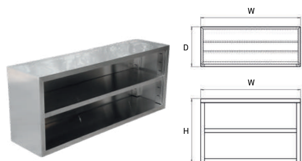
Open Wall Cabinet With Under Shelf
