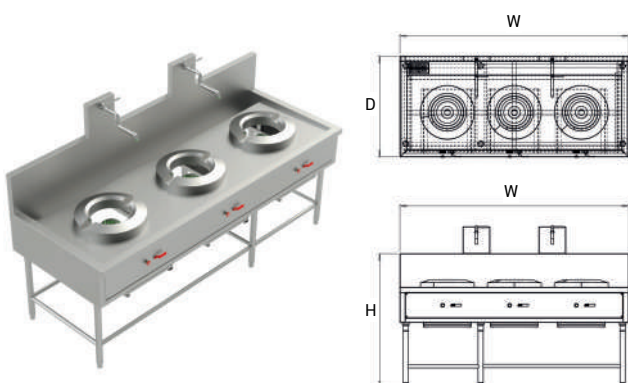
3-Burner Chinese Range With Faucet
