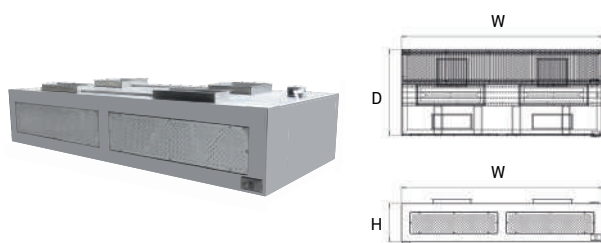
Hood
