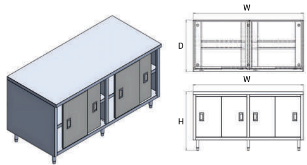
Cabinet Sliding Doors With Under Shelves
