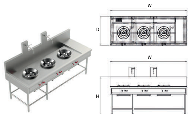
3-Burner Thai Range With Faucet
