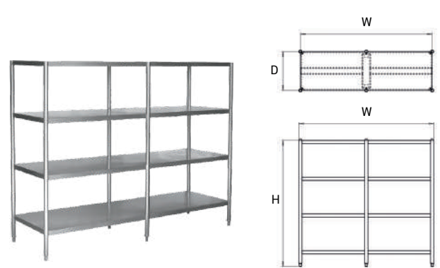
4 - Tiers Plain Shelves
