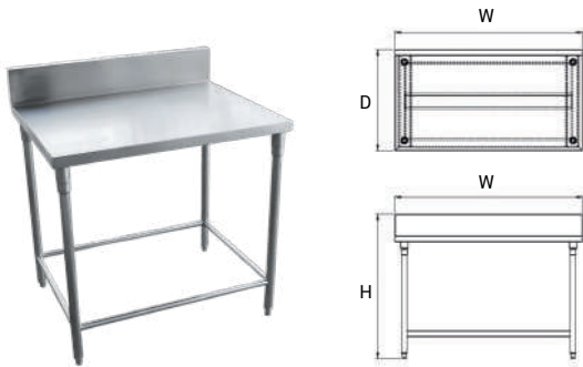
Work Table With Backsplash
