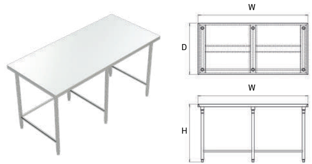
Work Table
